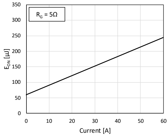
Fig. 15. E_{ON} vs. I_{DS} , T_{JUNC} = 25^\circ C
