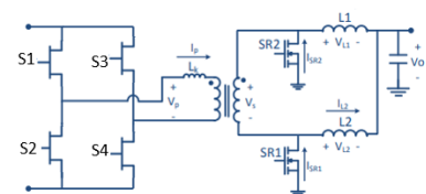
PSFB or DAB
